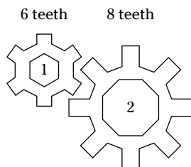
Figure 12-9: Ratio of teeth between two gears affects rotational speed.
