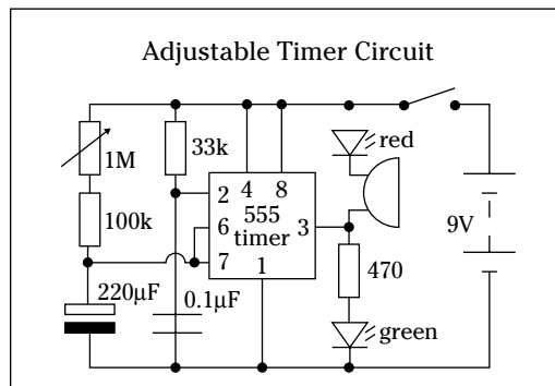
Figure 13-3: An adjustable timer circuit.
